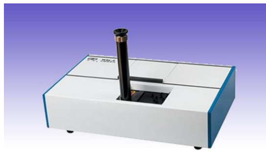
RS0046 Lovibond Tintometer Model SM-WSL2
